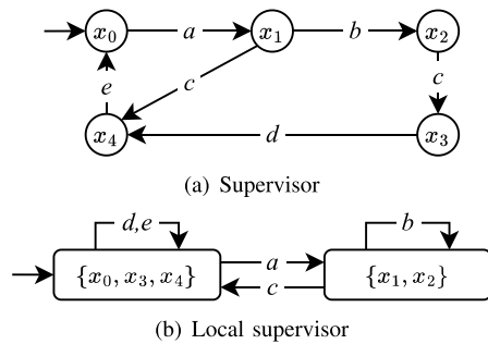
Fig. 1. Automata of Example 1.
