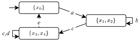
Fig. 2. Isolated state x_0 .
