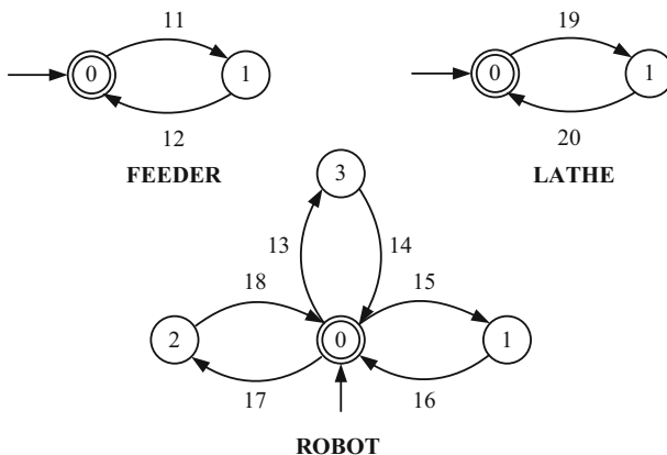
Fig. 12 Plant models to be controlled
